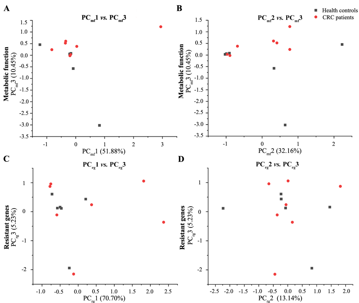
Fig. S1. Score plot results of metabolic function and resistant gene components PC1, PC2 and PC3. Metabolic function scores of A) PC mf 1 vs. PC mf 3 and B) PC mf 2 vs. PC mf 3; resistant gene scores of C) PC rg 1 vs. PC rg 3 and D) PC rg 2 vs. PC rg 3.
